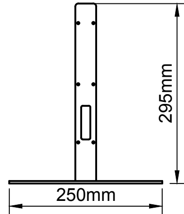
Front View (Scale1:6)
