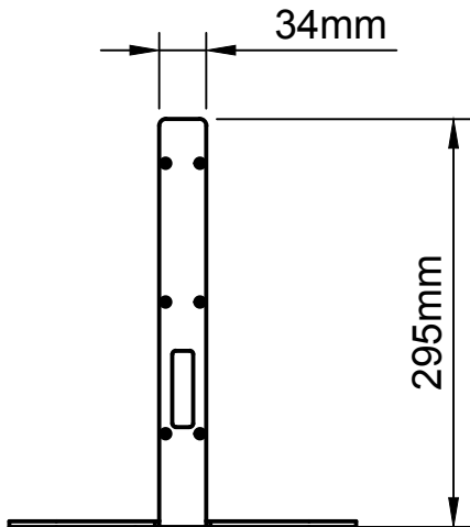
Rear View (Scale1:6)
